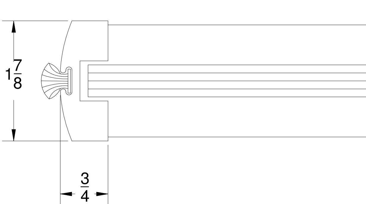
SECTION OF 3/4" VERTICAL STILE
