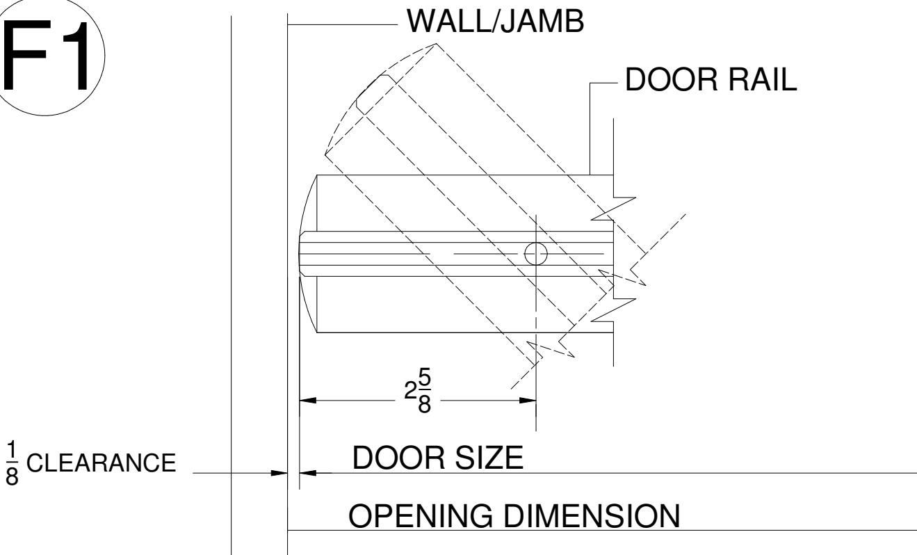
Door Edge Detail (Pivot Side) at Wall Type P or B/P Door
