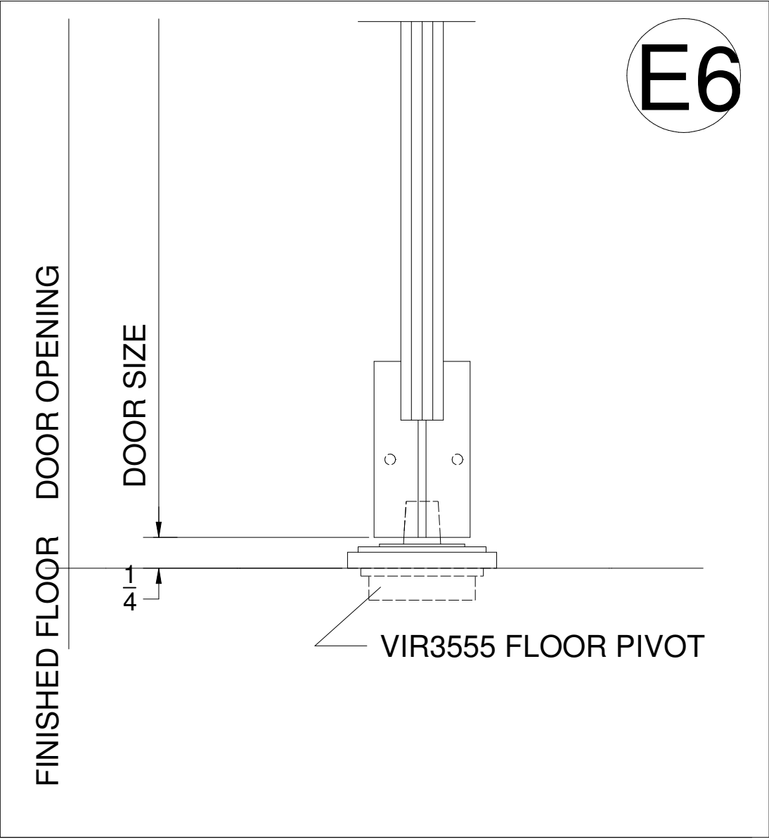
SILL DETAIL-Type AGA Door W/Floor Pivot
