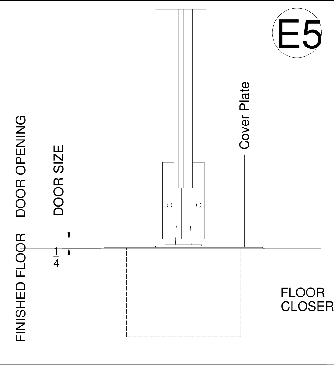
SILL DETAIL-Type AGA Door W/Floor Closer
