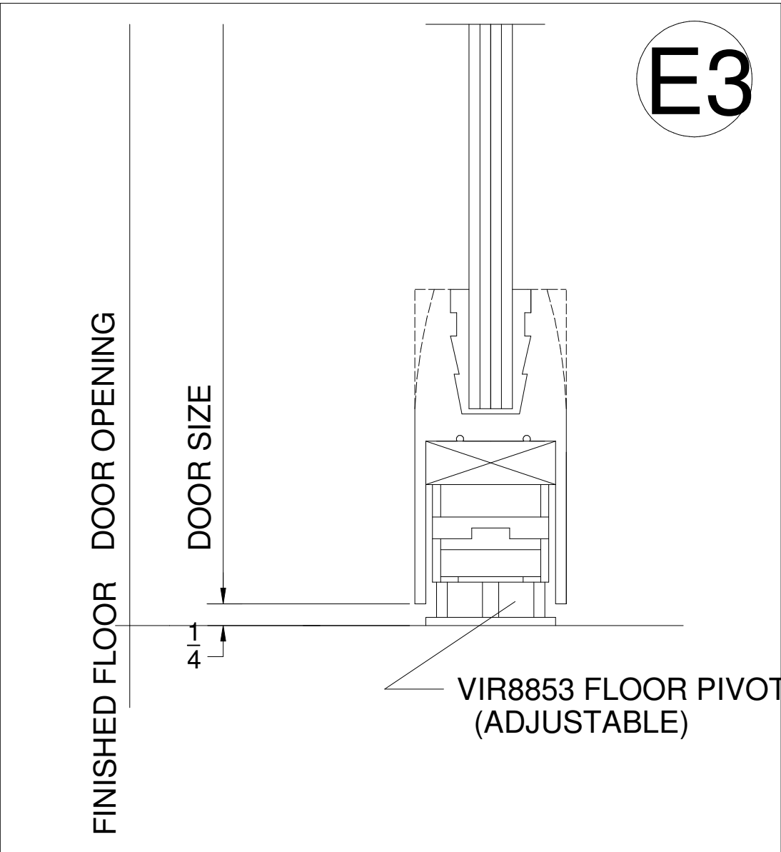
SILL DETAIL-Type P or B/P Door W/Floor Pivot
