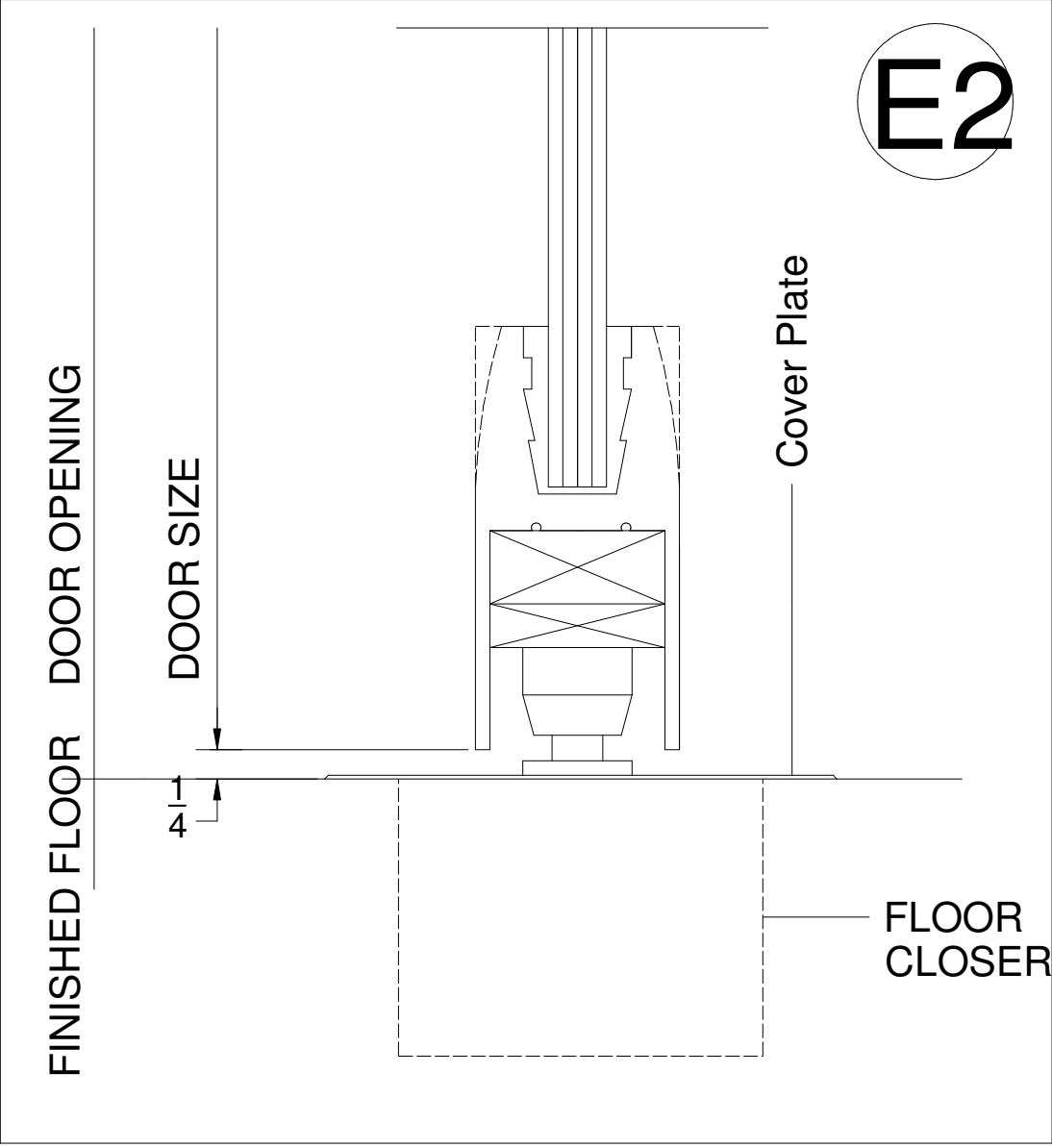
SILL DETAIL-Type P or B/P Door W/Floor Closer
