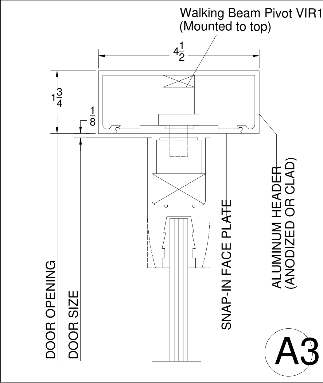
HEAD DETAIL-Type P Door W/Top Pivot
