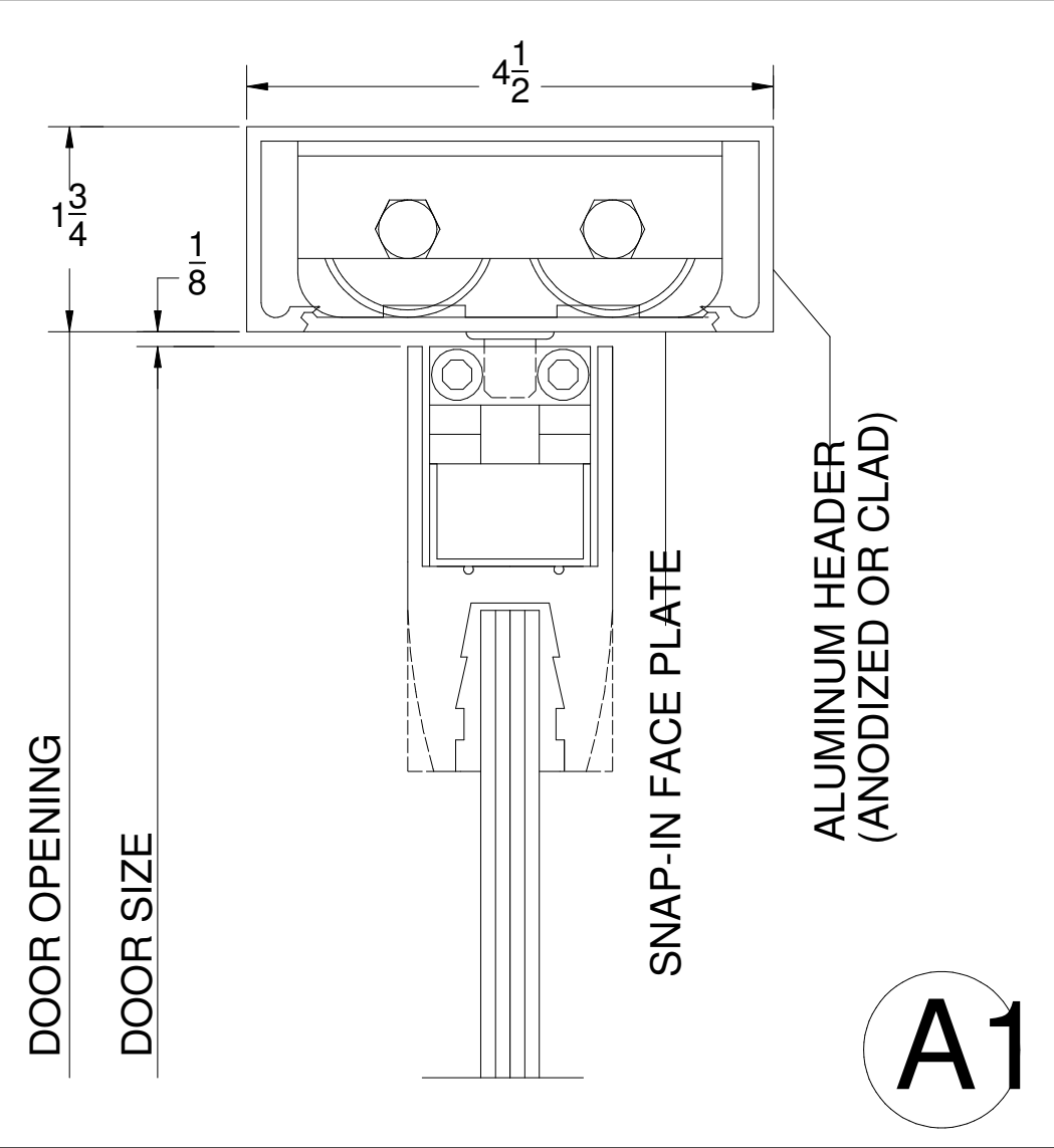
HEAD DETAIL-Type P Door W/Overhead Closer
